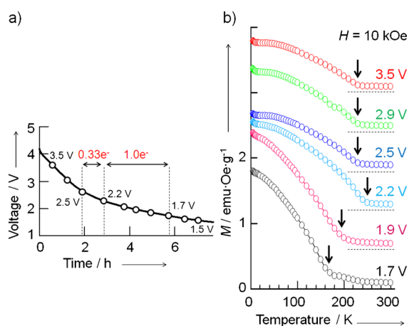
Figure 2. a) The first discharge curve of the mixed-valent chromium PBA battery. The open circles indicate the voltages at which magnetism was measured. b) Temperature dependence of the magnetization for the Cr PBA in the Li batteries at various voltages during discharge. The arrows, indicating quick rises in magnetization, are only guides for the eyes.
